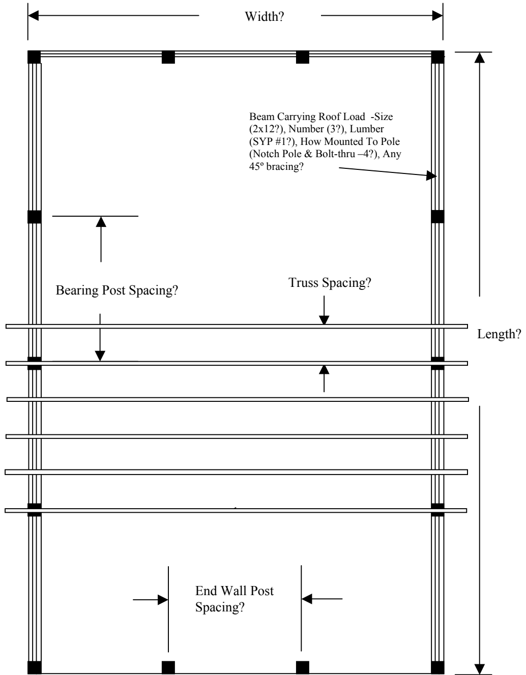
Plan View No Scale
